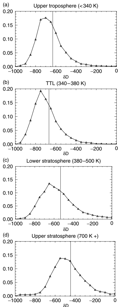
Figure 6. Distributions of values of \delta D in different atmospheric layers for the tropics and sub-tropics ( 30^{\circ}\text{S} – 30^{\circ}\text{N} ): (a) upper troposphere; (b) TTL; (c) lower stratosphere; and (d) upper stratosphere. Vertical lines denote the mean value of \delta D for each layer.
