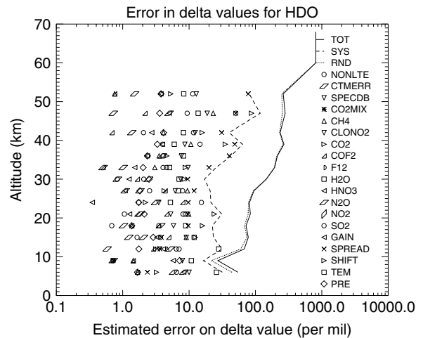
Figure 1. Estimated error components on δD for a single-profile retrieval, showing contributions from noise (RND) as well as from systematic (SYS) sources. Systematic error sources considered (shown by symbols) include contributions due to temperature, pressure and contaminant gases as well as instrumental effects and certain assumptions made in the forward model (Dudhia et al. , 2002). The instrumental effects considered are the radiometric gain (GAIN), the spectral shift (SHIFT) and uncertainties in the instrument line shape (SPREAD). Forward model errors considered include the assumption of local thermal equilibrium (NLTE), errors in the continuum (CTM) and uncertainties in the spectroscopic parameters (SPECDB). Temperature errors dominate the systematic error budget at the lowest altitudes. At higher altitudes, the dominant systematic errors are the uncertainties in the spectral shift and the instrument line shape.
