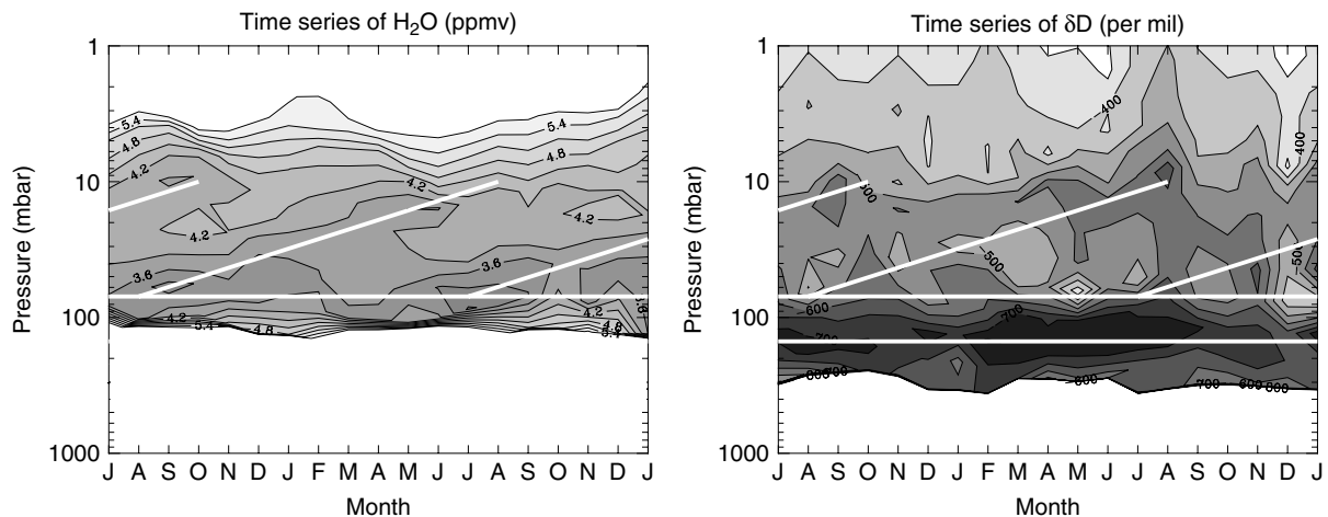
Figure 8. Time series of mean H_2O and \delta D in the tropics. Horizontal lines denote the approximate boundaries of the TTL at 150 and 70 mbar. Sloping lines on both plots represent the ascent of dry air upwards (the ‘tropical tape recorder effect’). Contour intervals are 0.3 ppmv for H_2O and 50‰ for \delta D .
