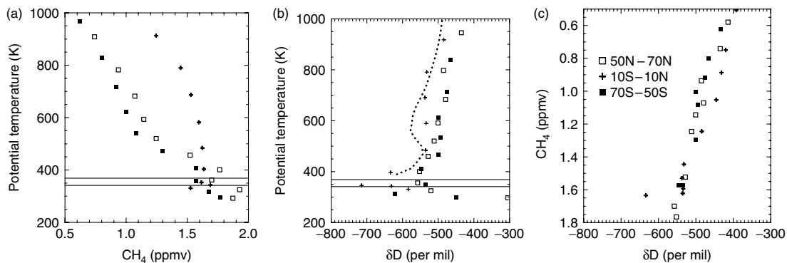
Figure 5. (a) Zonal annual mean profiles of CH_4 from three latitude bands, showing evidence of ascending motion in the tropics and descending motion at higher latitudes. (b) Zonal annual mean profiles of \delta D from three latitude bands, showing the large depletion in the tropical upper troposphere, the sharp gradient in the TTL and mixing in the stratosphere. The dotted line shows the theoretical gradient profile that would result from formation of stratospheric water vapour from the oxidation of methane and molecular hydrogen. (c) Scatter plot of \delta D and CH_4 in the stratosphere (points above 380 K). Means for this figure were all calculated using data processed for 2003.
