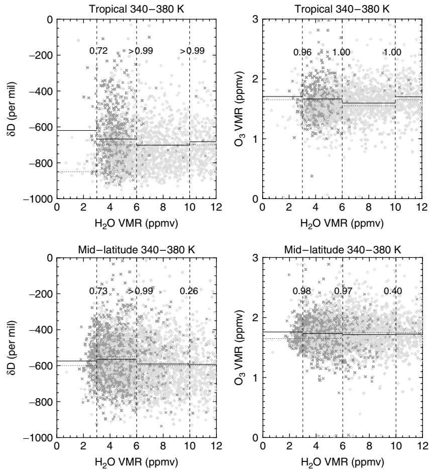
Figure 7. Scatter plots showing \delta D (left) and O_3 (right) as a function of water vapour in the TTL (340–380 K) and in the same potential temperature layer at mid-latitudes. Lighter diamonds show points with potential temperatures in the range 340–360 K (the lower altitude range of the layer), while darker crosses show points with potential temperatures in the range 360–380 K (the upper part of the layer). Solid horizontal lines show mean \delta D (left) and O_3 (right) values in selected H_2O bins, denoted by vertical dashed lines. Numbers associated with these dashed vertical lines show the confidence levels (to two decimal places, from a t -test) that the means in adjacent bins are statistically different. A value of 1.00 implies that the confidence level is greater than 99%. Dotted horizontal lines show the median value in each of the H_2O bins.
